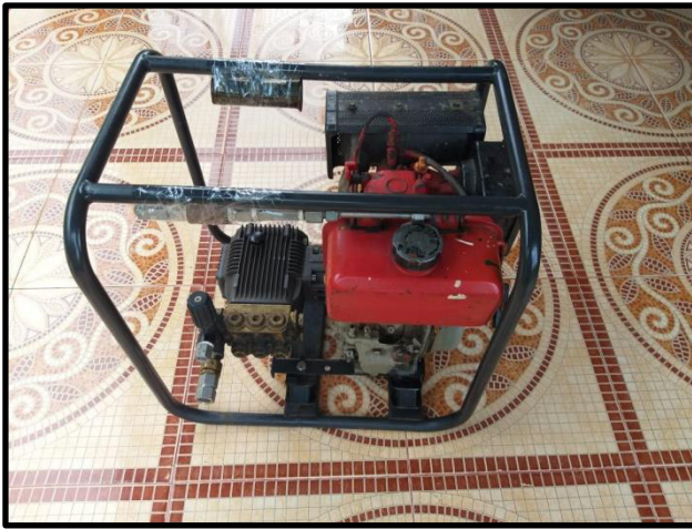
ENGINE PUMP @ 35 LITER / MINUTES MAX PRESSURE 5000 PSI
